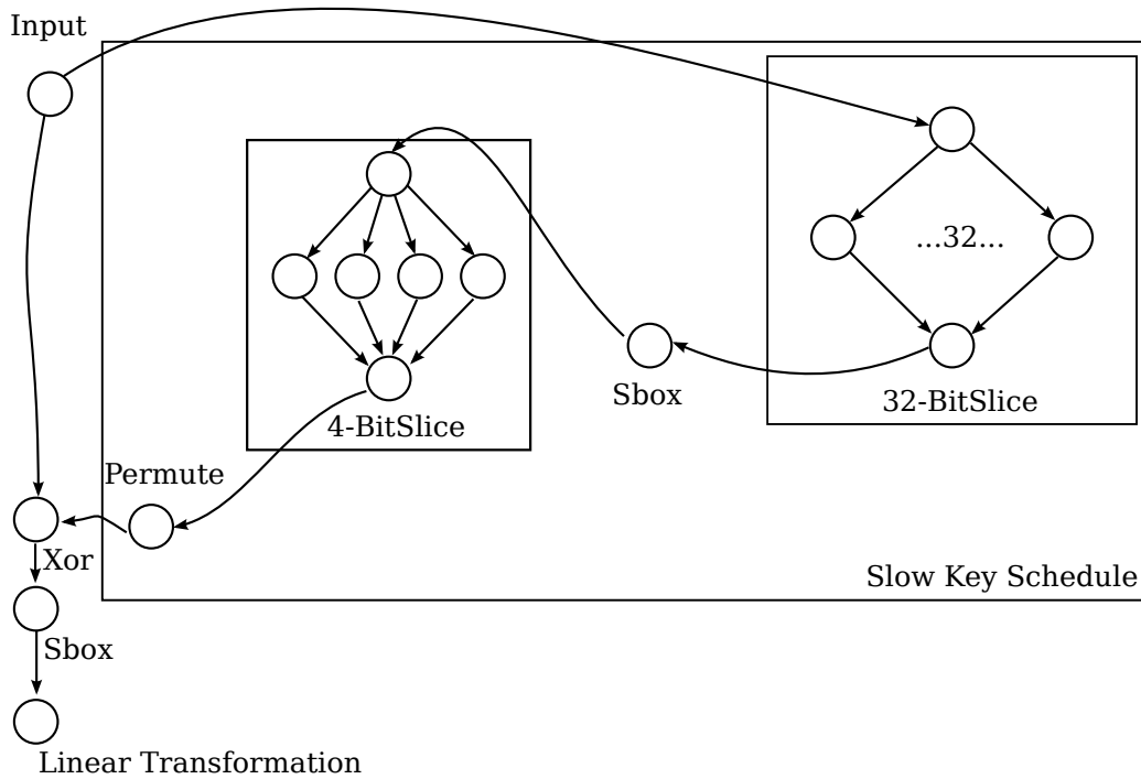
Figure 4.1 One round in the Serpent encryption algorithm
